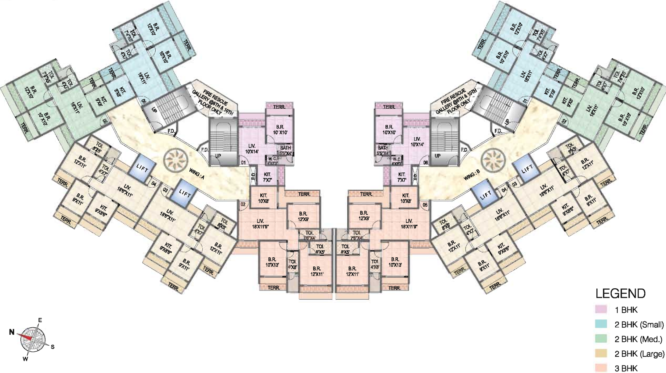
Typical Even Floor Plan (4th/6th/8th/10th/12th Floor)
